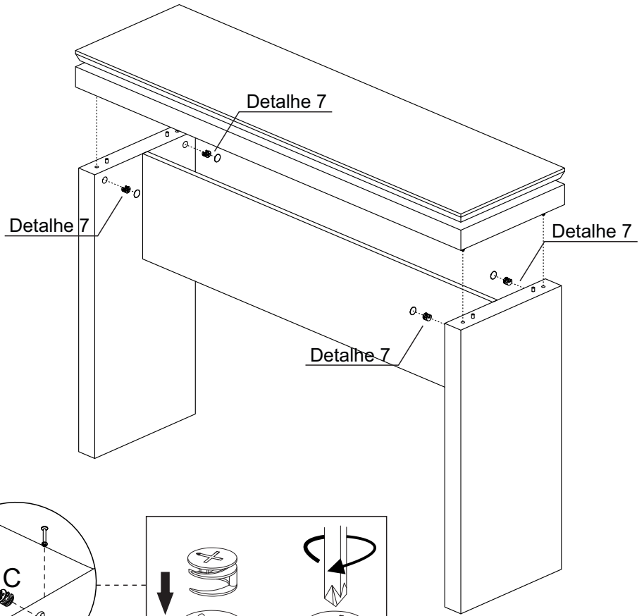
Detalhe 7 Detalle/Detail
