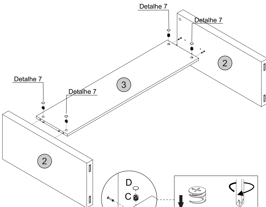
Detalhe 7 Detalle/Detail
