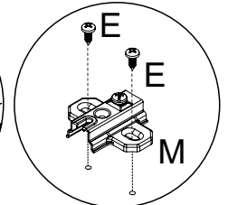
Detalhe 3 Detalle/Detail
