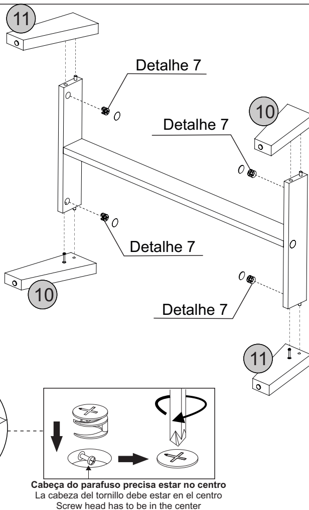
Detalhe 7 Detalle/Detail
