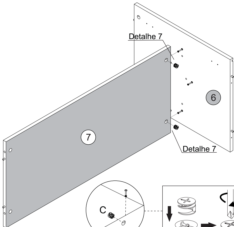
Detalhe 7 Detalle/Detail
