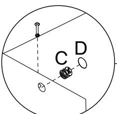
Detalhe 12 Detalle/Detail
