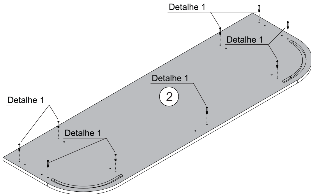
Detalhe 1 Detalle/Detail
