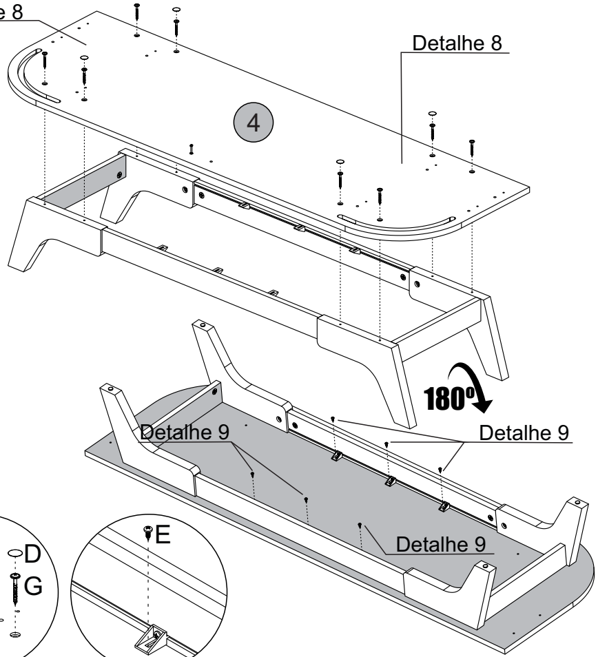
Detalhe 9 Detalle/Detail
