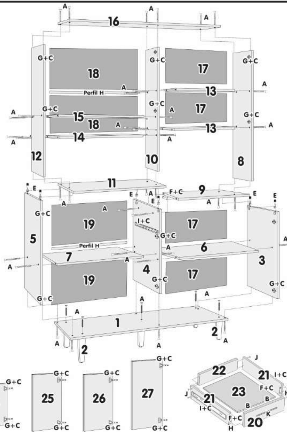
F - Cantoneira 4 Furos
