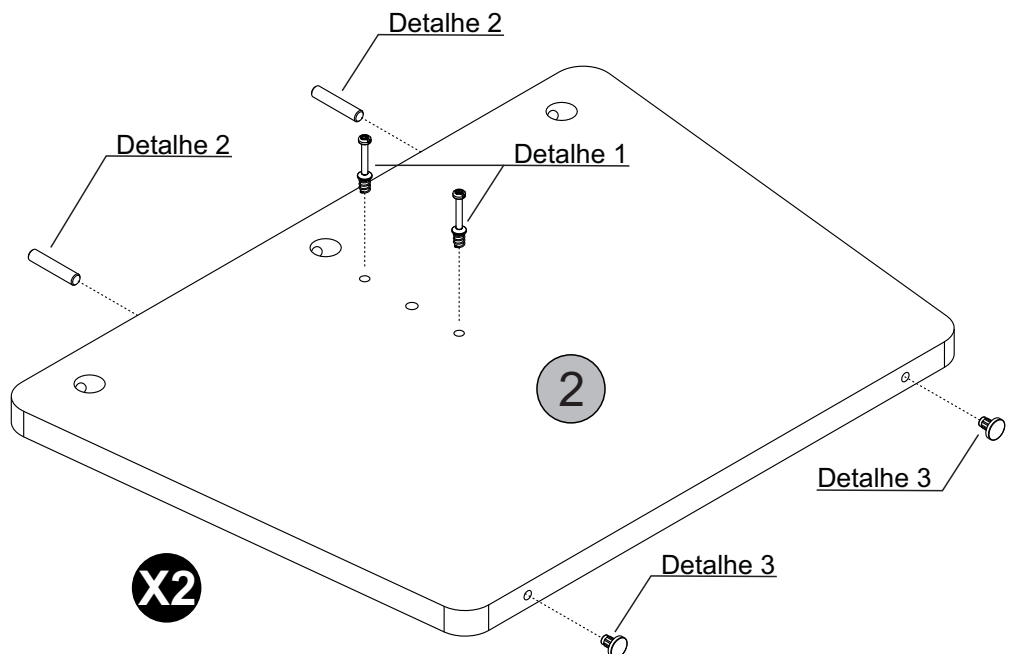
Detalhe 1 Detail/Detaille
