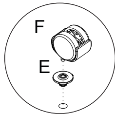
Detalle 1 Detalle/Detail
