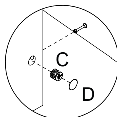
Detalle 5 Detail/Detalle
