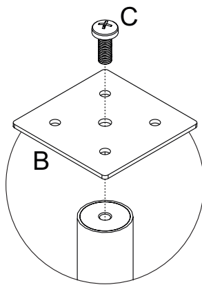
Detalhe 2 Detalle/Detail
